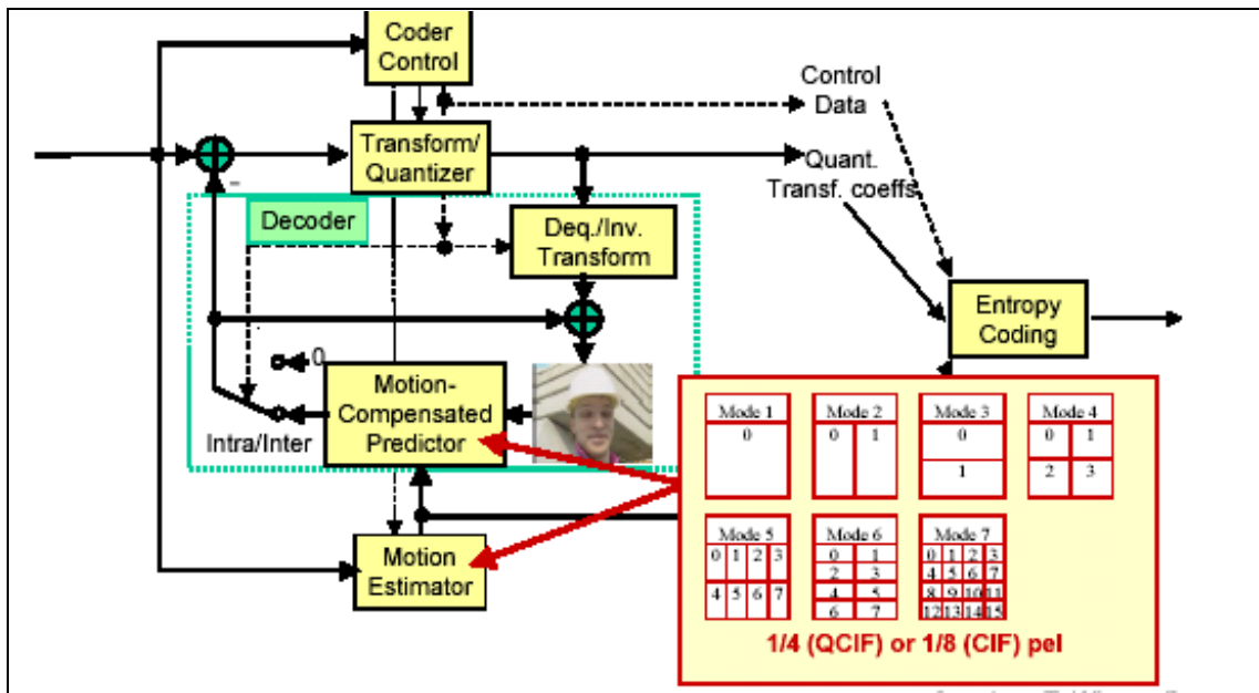
Figure 3. Macroblock division
