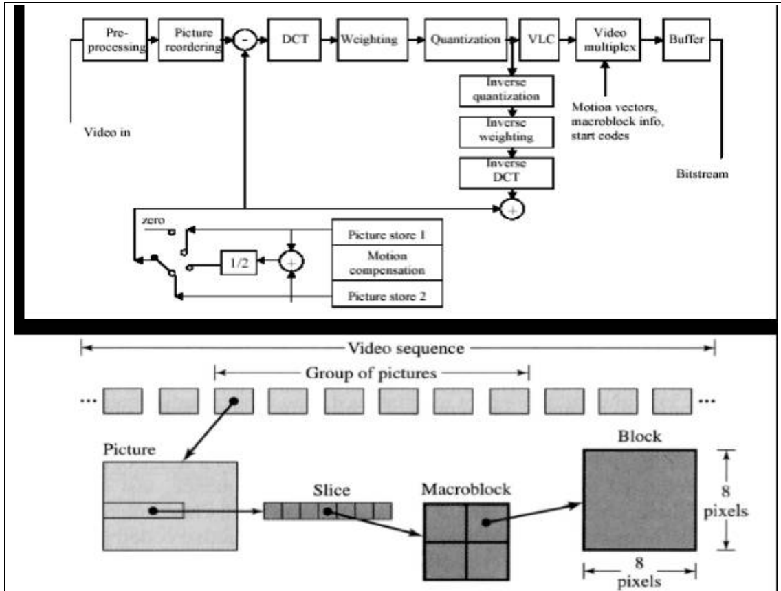
Figure 2. MPEG-2 encoding
